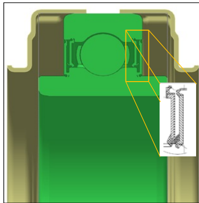
Figure 1. Sectioned view of the centre bearing (seal lip area enlarged)
